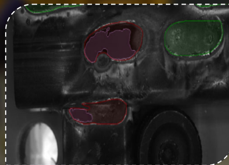
Weld inspection
